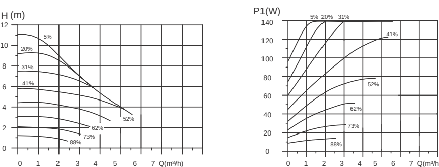
RCE 25-11 Series Performance Chart (PWM)
