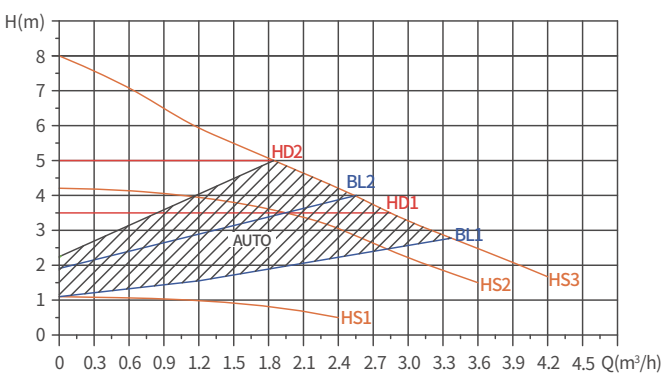
REXX-8 Performance curves
