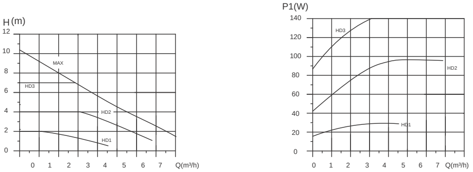
RCE 32-11 Series Performance Chart (Constant Pressure)
