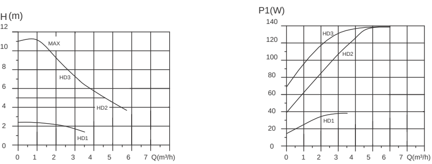
RCE 25-11 Series Performance Chart (Constant Pressure)
