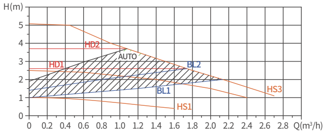
REXX-5 Performance curves
