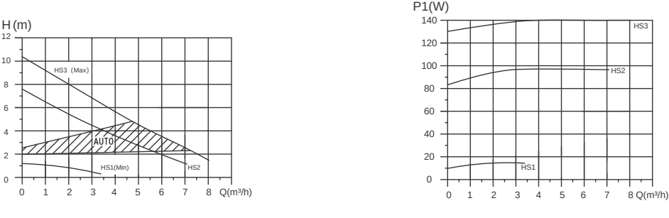
RCE 32-11 Series Performance Chart (Constant Speed+Auto Mode)
