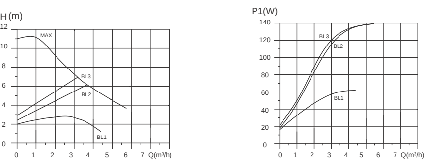
RCE 25-11 Series Performance Chart (BL Mode)
