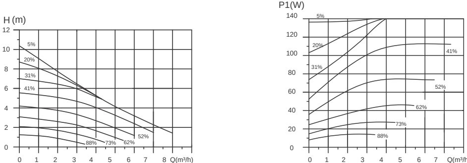
RCE 32-11 Series Performance Chart (PWM)
