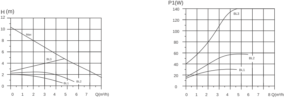
RCE 32-11 Series Performance Chart (BL Mode)
