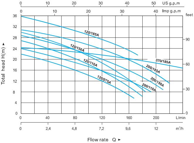
PERFORMANCE CHART AT n=2900 r/min
