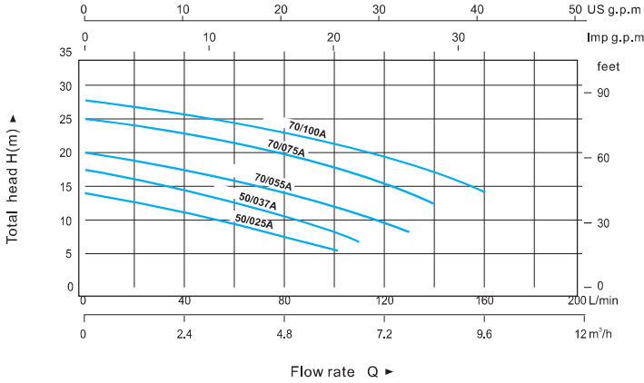
PERFORMANCE CHART AT n=2900 r/min
