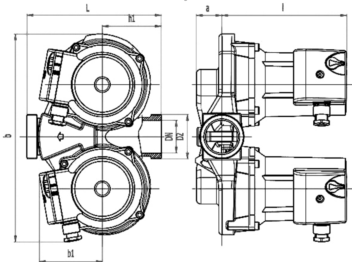
Dimension drawing
