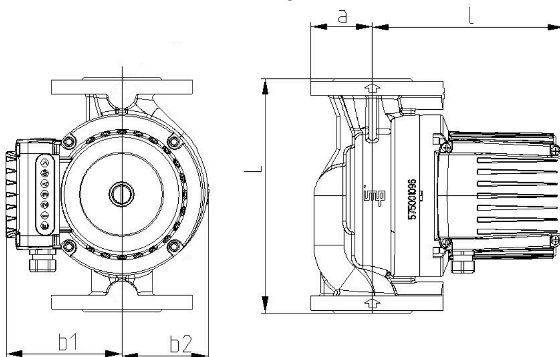
Dimension drawing
