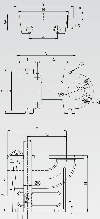
Fixed Part for Guide Tube
